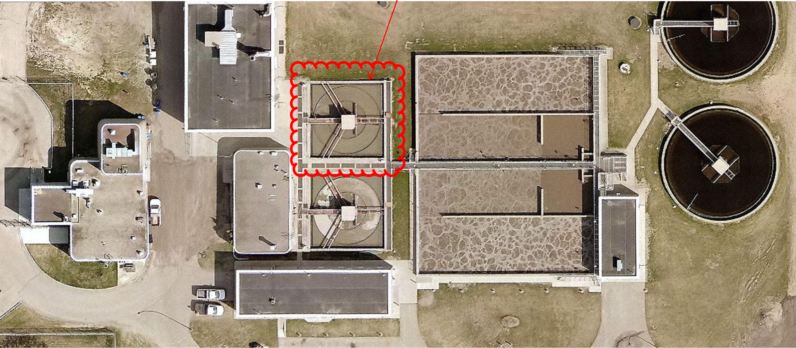
North Primary Clarifier
